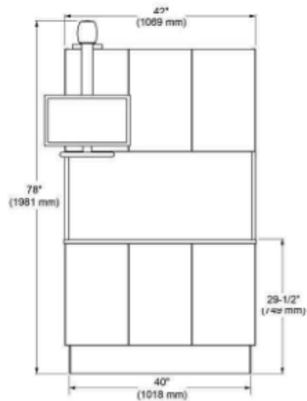
391 Elevation Front
