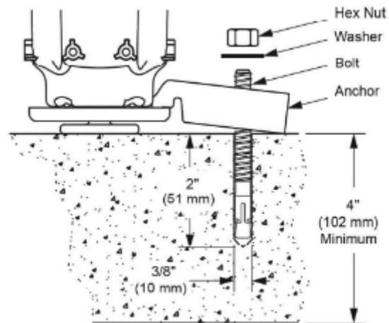
Concrete Floor Anchor
