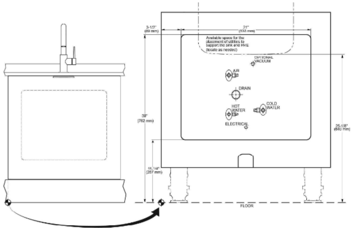
Utility Layout Detail - Sink Module
