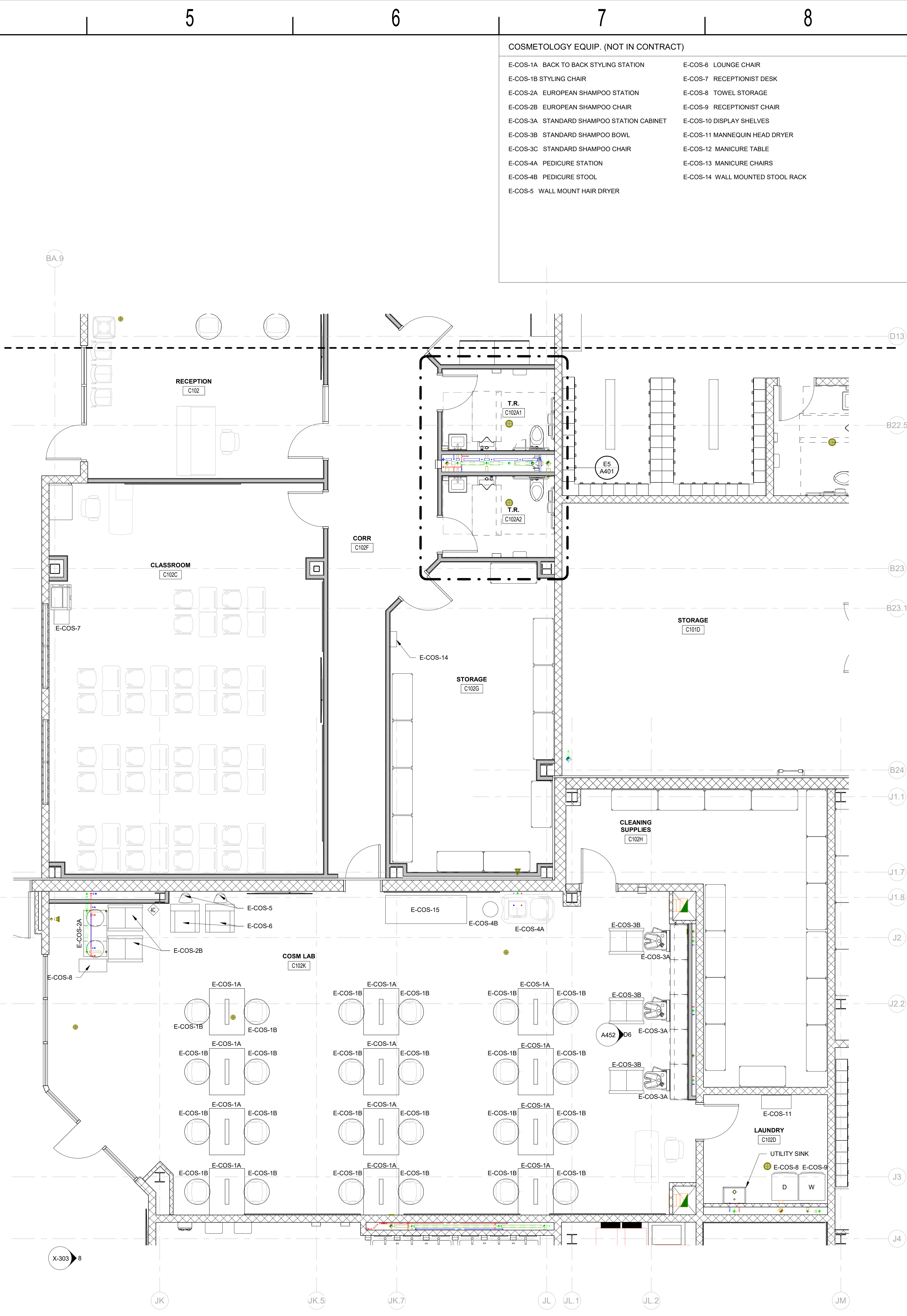
A4 ENLARGED PLAN - FIRST FLOOR - KEYPLAN 10 - COSMETOLOGY 1/4" = 1'-0"
