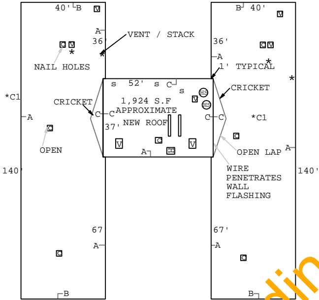
BUILDING T-2 (5,563 S.F. APPROXIMATE)
