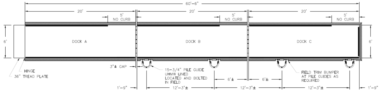
OVERALL PLAN x2 SCALE: 1/4"=1'-0" ONE AS SHOWN, ONE MIRRORED
