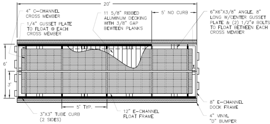
DOCK A DETAIL SCALE: 1/4"=1' ONE AS SHOWN, ONE MIRRORED
