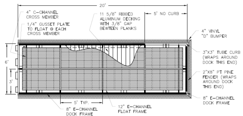
DOCK C DETAIL SCALE: 1/4"=1' ONE AS SHOWN, ONE MIRRORED
