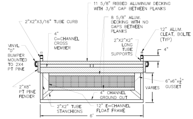
DOCK SECTION SCALE: 1/2"=1'-0"
