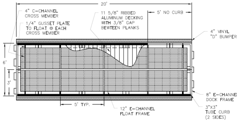
DOCK B DETAIL SCALE: 1/4"=1' ONE AS SHOWN, ONE MIRRORED
