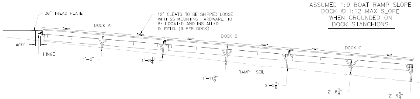
ELEVATION x2 SCALE: 1/4"=1'-0" (SHOWN FULLY GROUNDED)
