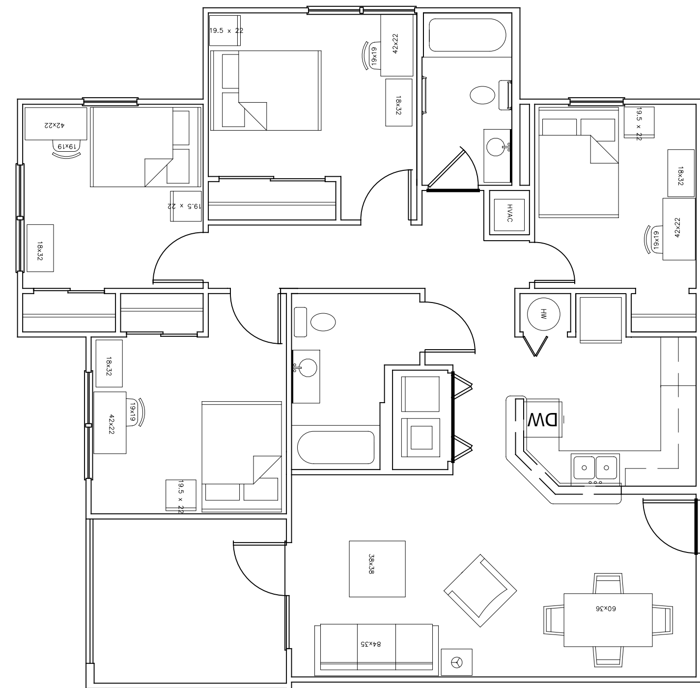
2 A-1 UNIT TYPE D.4HC, TYP. PLAN SCALE: 3/16" = 1'-0" UNIVERSITY COURTYARD
