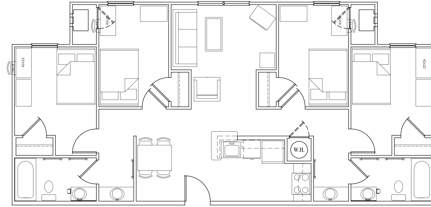
4 A-2 UNIT TYPE D-2, TYP. PLAN SCALE: 3/16" = 1'-0" UNIVERSITY VILLAGE
