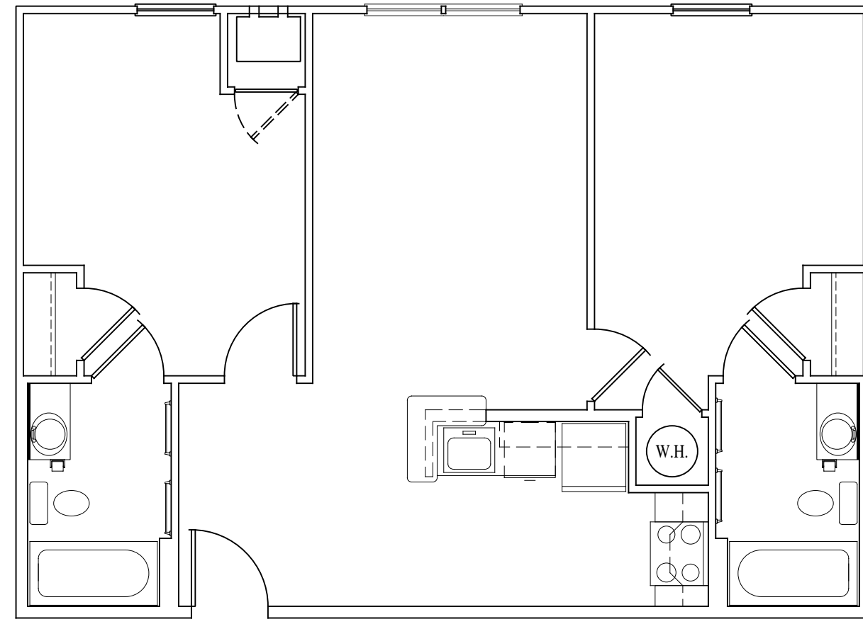
1 A-2 UNIT TYPE B-2, TYP. PLAN SCALE: 3/16" = 1'-0" UNIVERSITY VILLAGE
