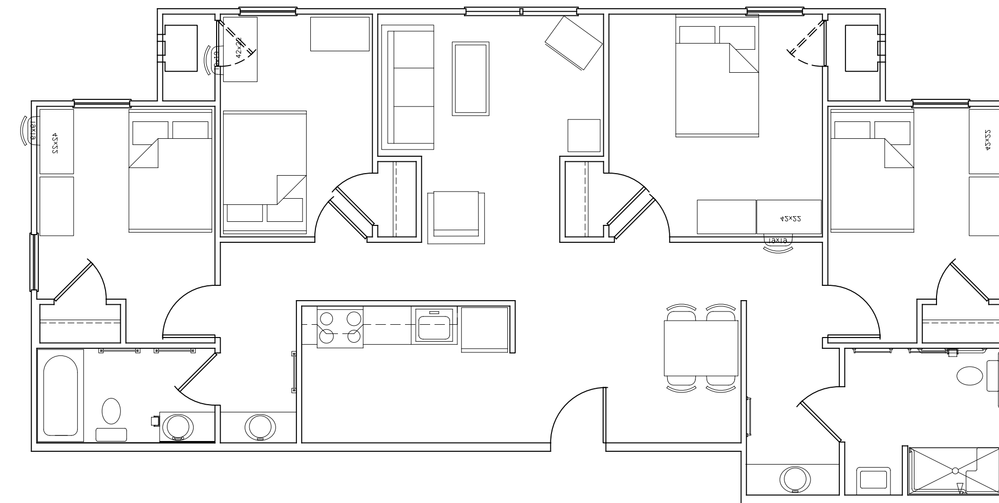
6 A-2 UNIT TYPE D-2HC, TYP. PLAN SCALE: 3/16" = 1'-0" UNIVERSITY VILLAGE
