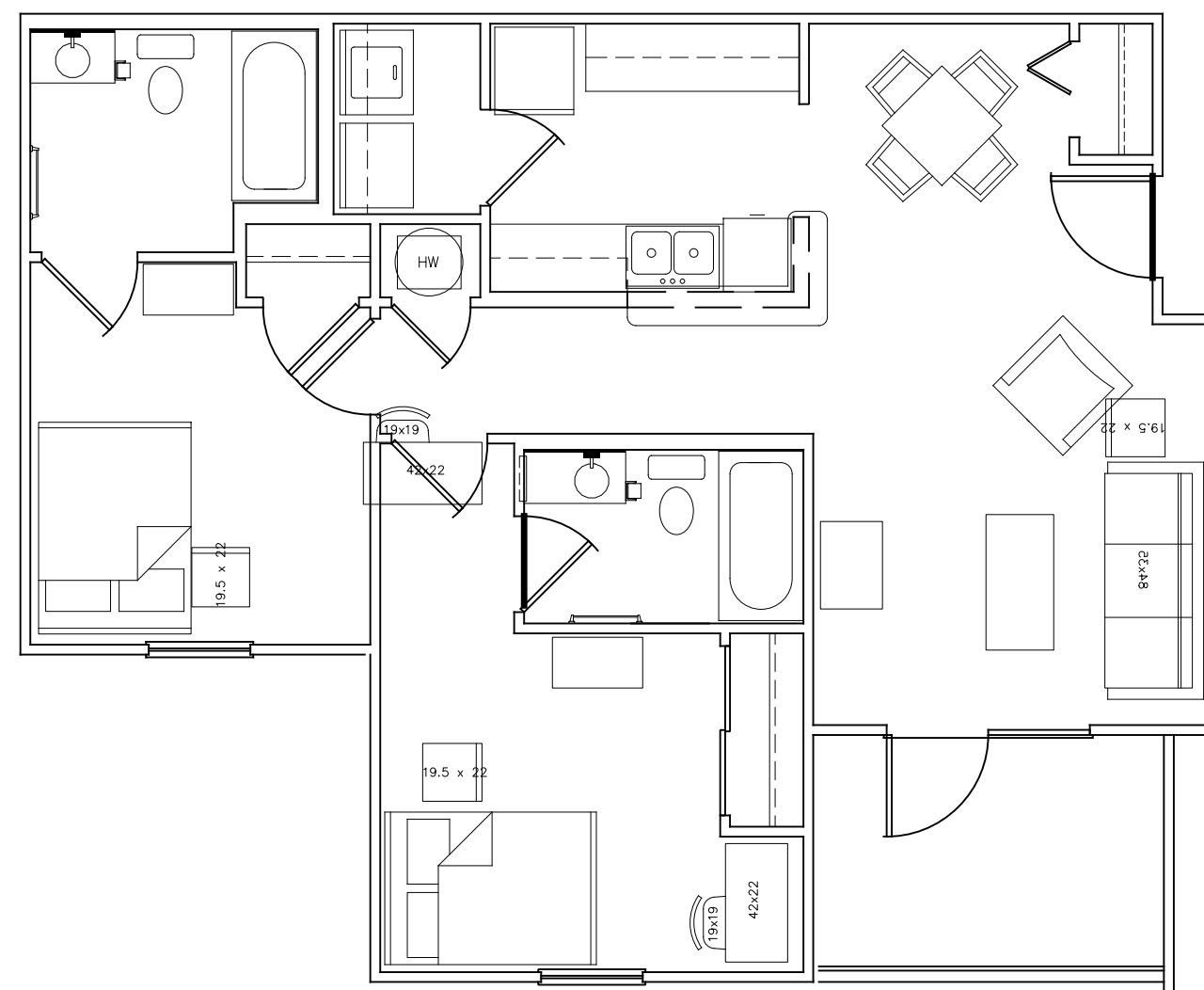
4 A-1 UNIT TYPE B.2HC, TYP. PLAN SCALE: 3/16" = 1'-0" UNIVERSITY COURTYARD
