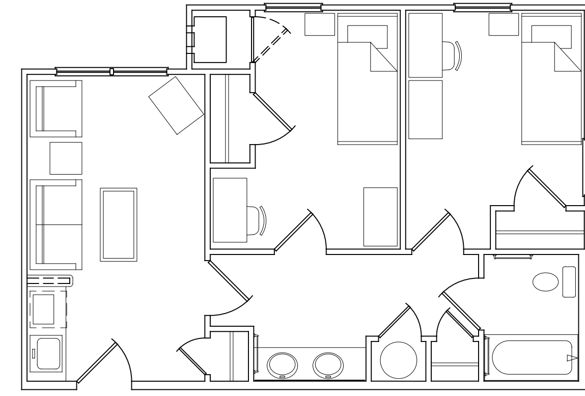
7 A-1 UNIT TYPE B-1A, TYP. PLAN SCALE: 3/16" = 1'-0" UNIVERSITY VILLAGE
