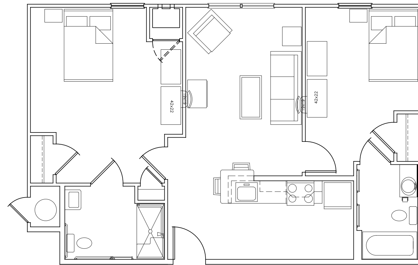
3 A-2 UNIT TYPE B-2HC, TYP. PLAN SCALE: 3/16" = 1'-0" UNIVERSITY VILLAGE
