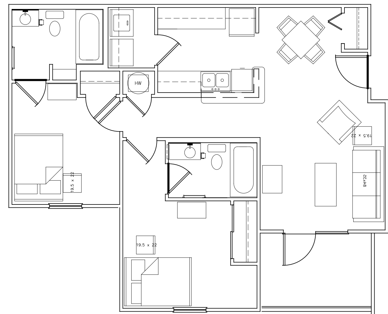
3 A-1 UNIT TYPE B-2, TYP. PLAN SCALE: 3/16" = 1'-0" UNIVERSITY COURTYARD
