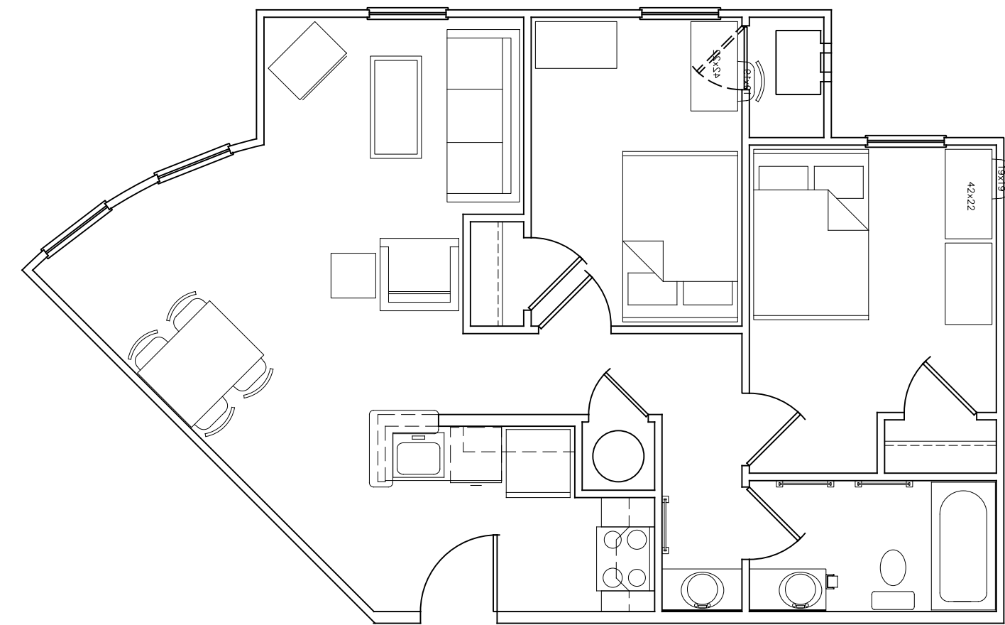
2 A-2 UNIT TYPE B-2A, TYP. PLAN SCALE: 3/16" = 1'-0" UNIVERSITY VILLAGE
